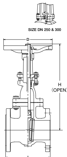
Fig. PN16FCL
